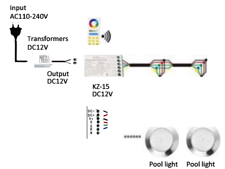
Wiring diagram of pool light
