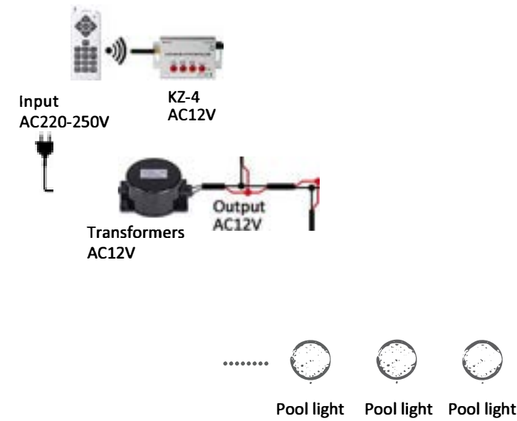
Wiring diagram of pool light
